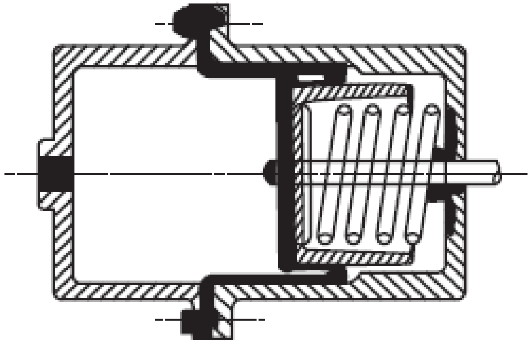
FIGURE 16-12 Diaphragm seals-rolling diaphragm.
